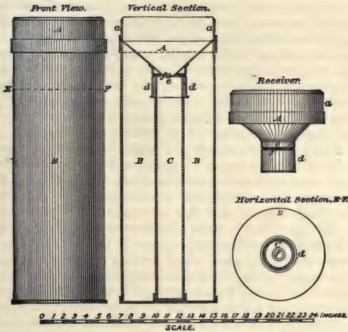
FIGURE 14. Rain-gauge.
